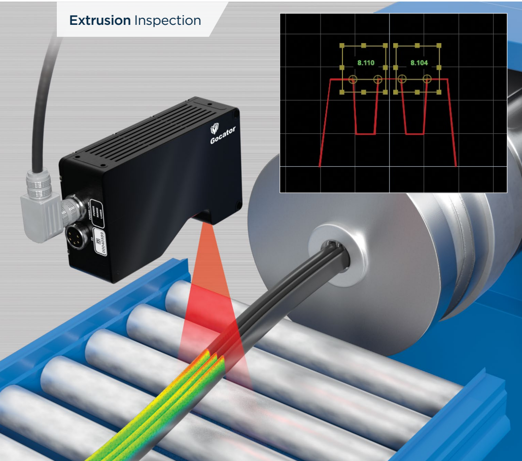
Laser line measurement of a plastic extrusion to ensure the correct spacing between teeth
