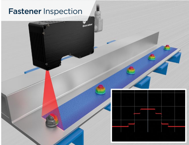
Checking the tightness of a fastener through measurement of mating surface to nut surface
