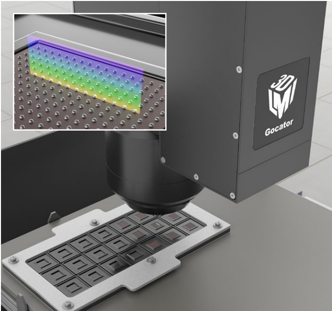
BGA Ball Bump Measurement
