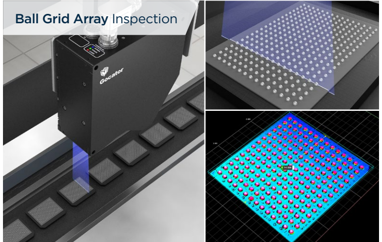
BGA Ball Bump Inspection using a Gocator 6320. Telecentric line generation improves small defect and edge detection.
