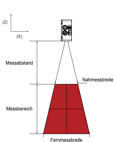
Gocator 2430
