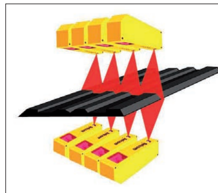
Eight sensors are used for the in-process profiling application to provide high data density across the full width of the extrusion
