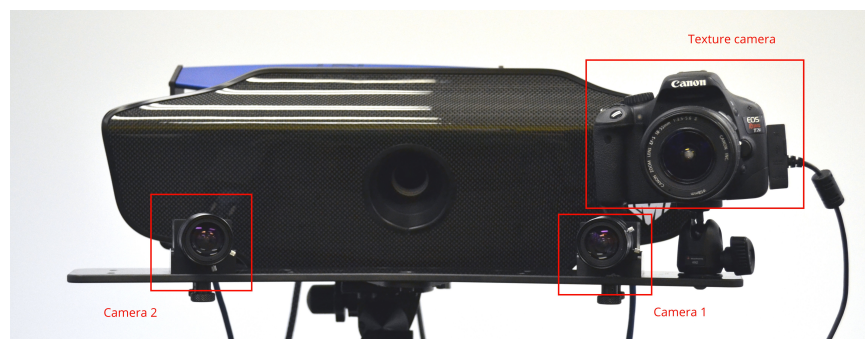
Texture camera setup
